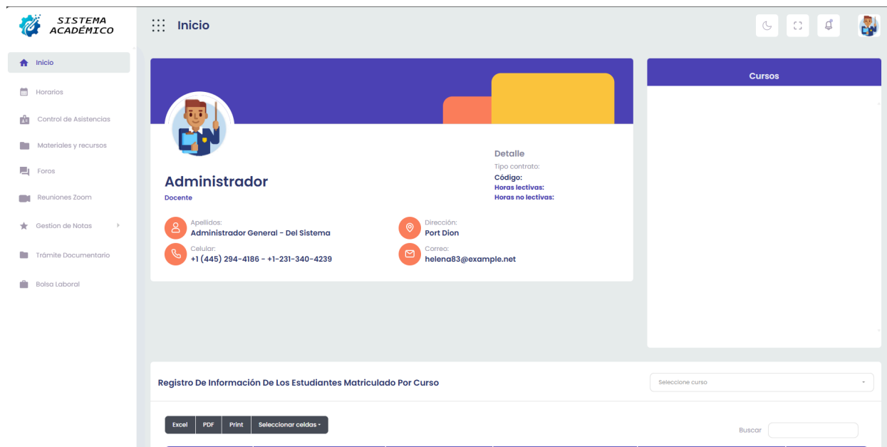
Figura 2. Dashboard
